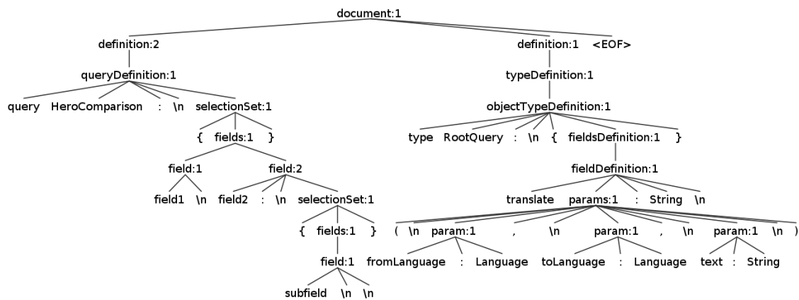
Figure 2. RCCN Parse Tree
